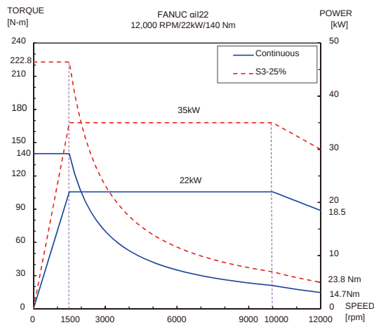
12,000rpm Direct drive spindle (OPT:H16)
