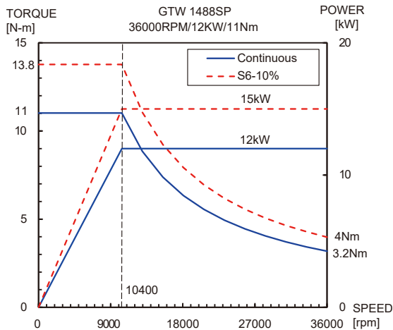
36,000rpm GTW Built-in spindle (ST:H6) 12/15 kW Power (Cont./S6-10%) 11/13.8 N.m Torque (Cont./S6-10%)
