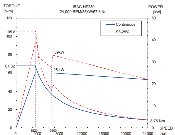
24,000rpm IBAG Built-in spindle (OPT:H16) 25/39 kW Power (Cont./S3-25%) 67.82/105.8 N.m Torque (Cont./S3-25%)
